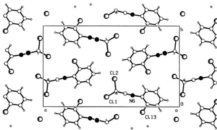
Fig. 4. Projection of the unit cell of o -ClPhDCA along [100].
